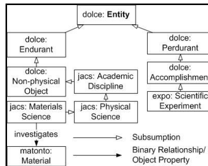
Figure 3: Materials Science Extensions to the Top-level Classes
