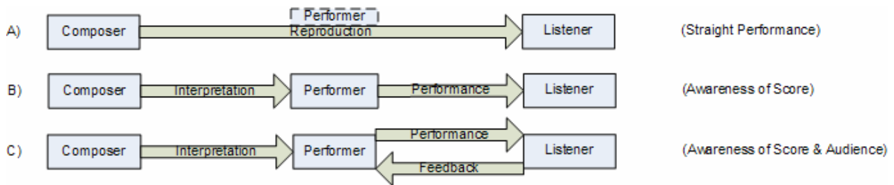
Figure 1. Performance Models
