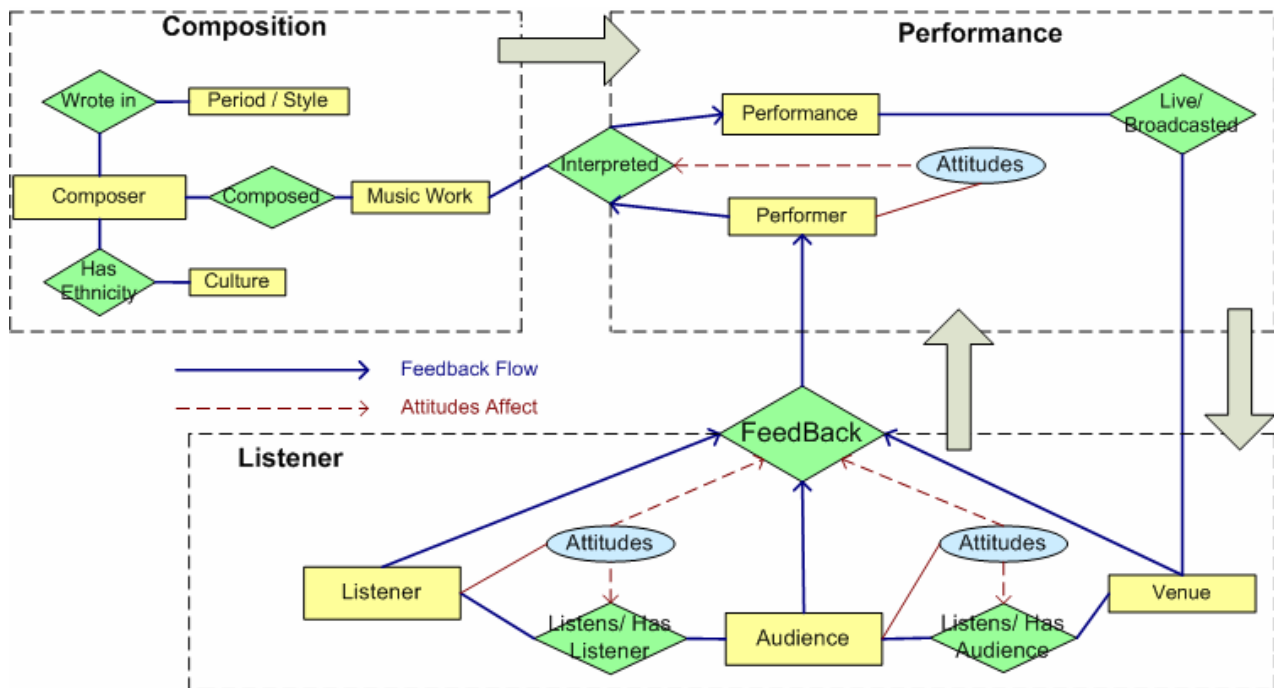
Figure 2. Music Environment
