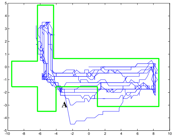
Figure 8. RatSLAM trajectory – unique landmarks.
